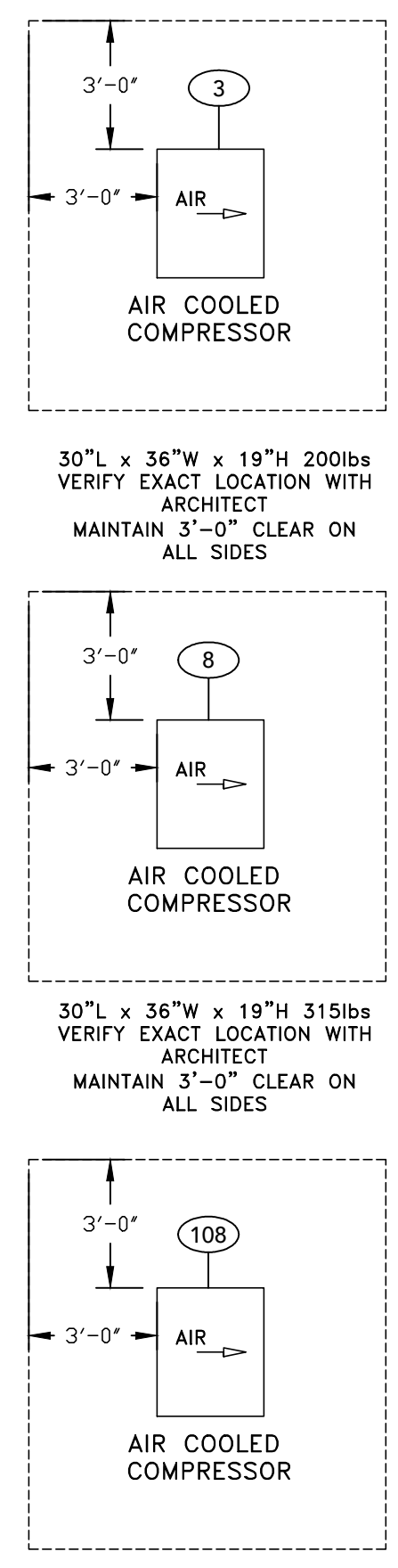
1 FOODSERVICE EQUIPMENT PLAN Scale: 1/4"=1'-0"
