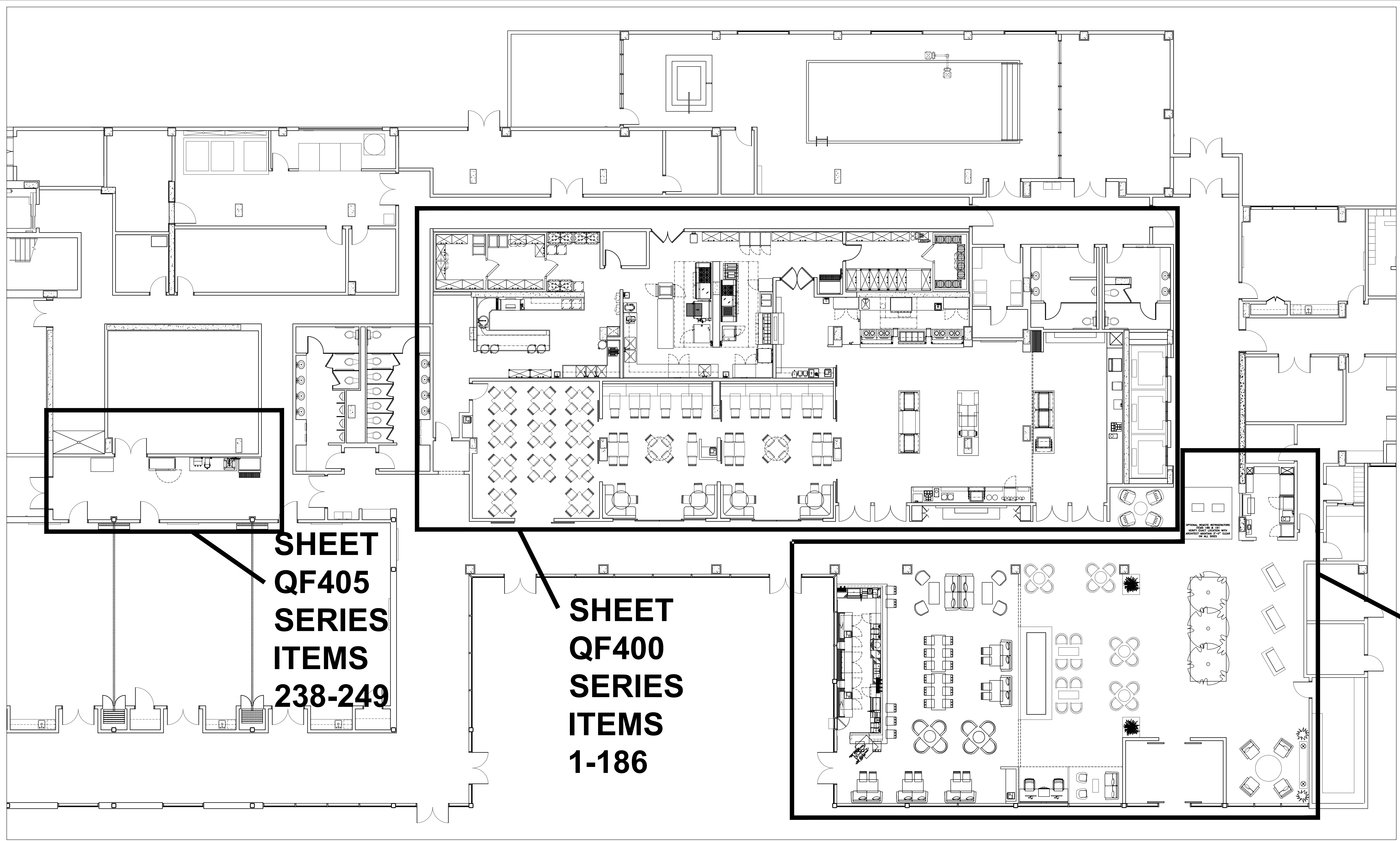
1 FOODSERVICE OVERALL PLAN Scale: 1/8"=1'-0"
