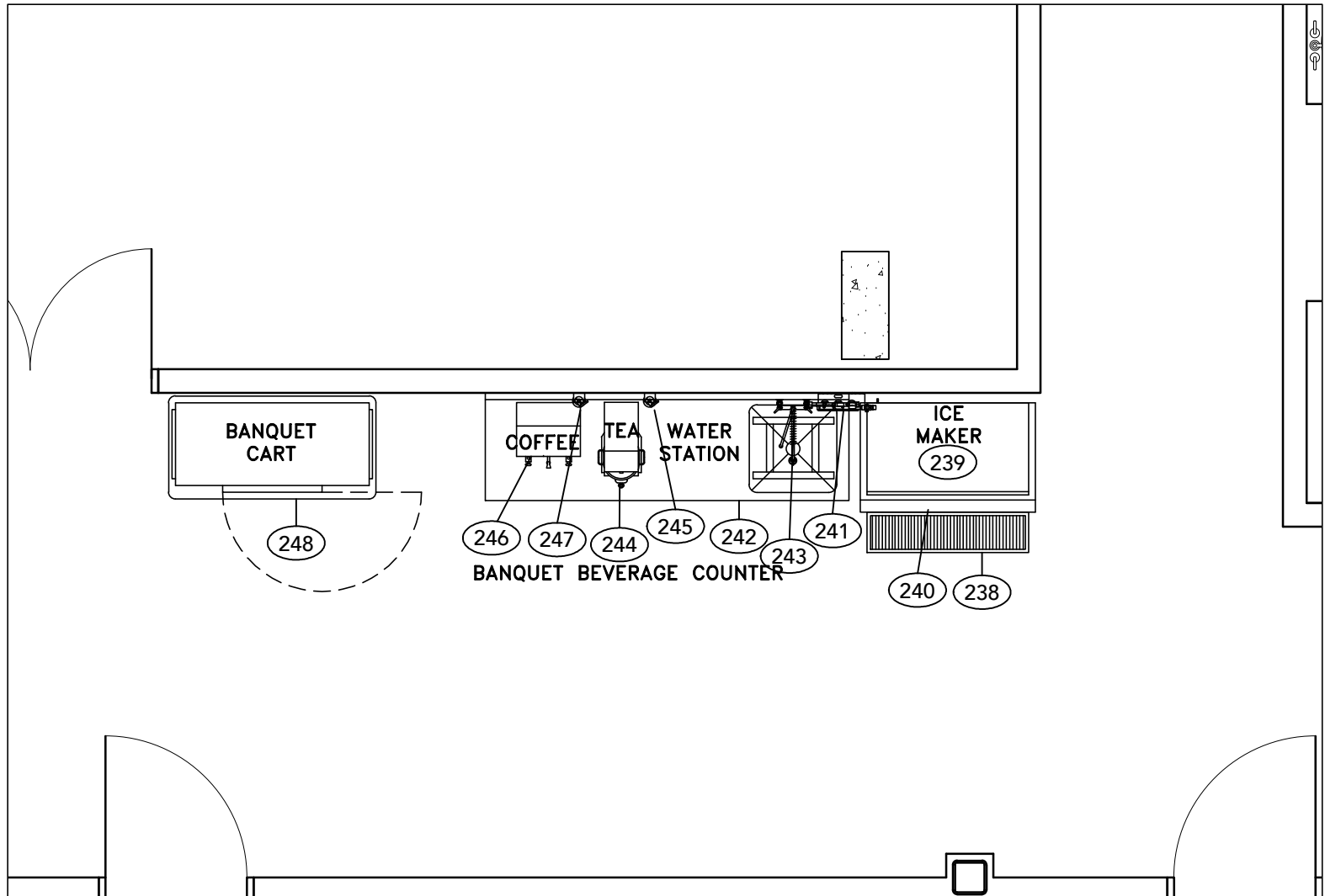
1 FOODSERVICE EQUIPMENT PLAN Scale: 1/4"=1'-0"
