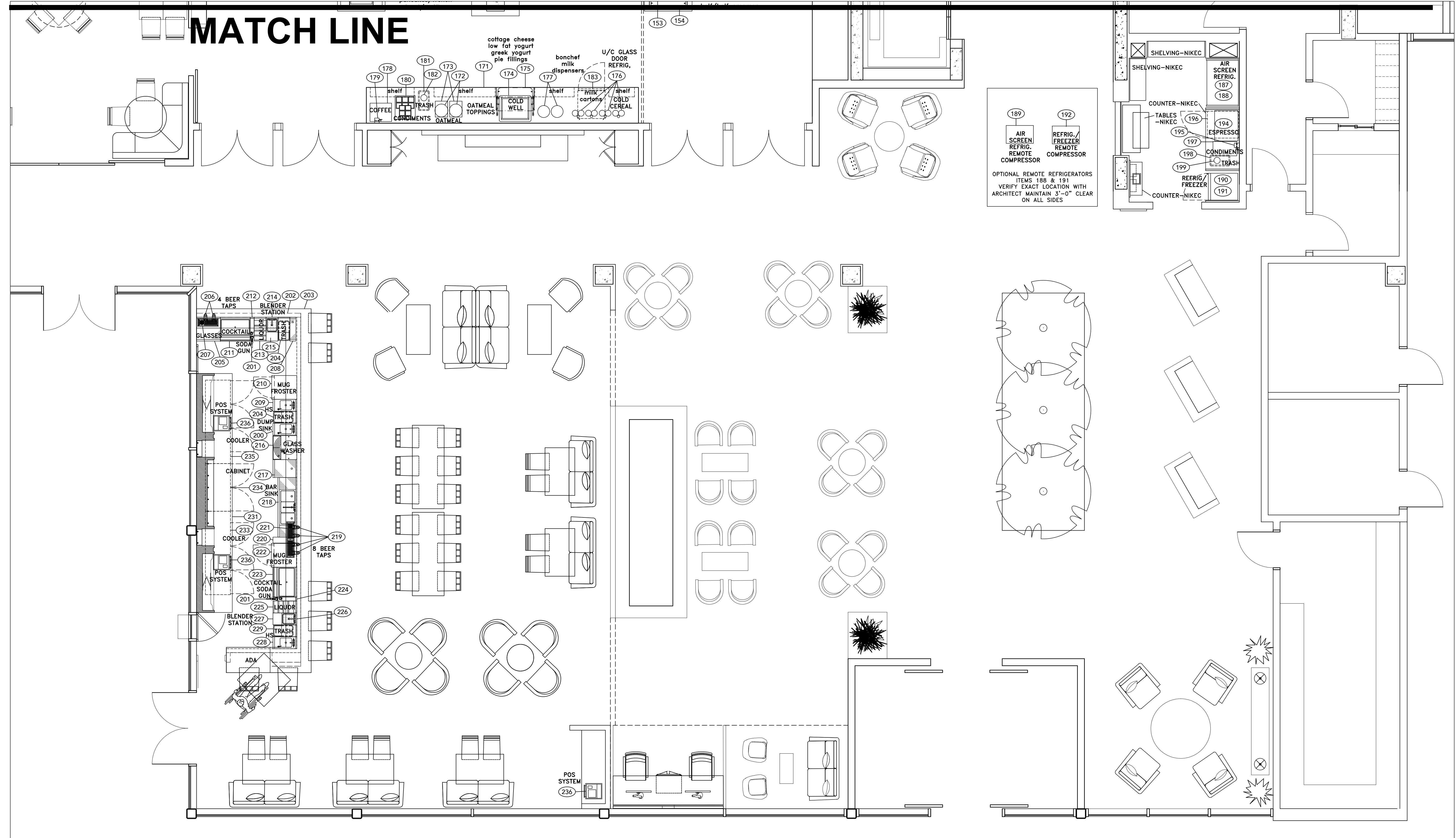
2 FOODSERVICE EQUIPMENT PLAN Scale: 1/4"=1'-0"
