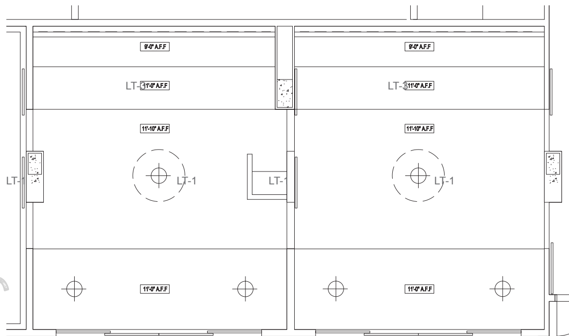
REFLECTED CEILING PLAN
