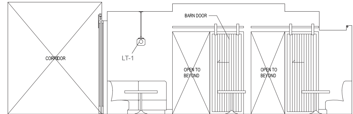
ELEVATION-VIEW FROM DINING ZONE 2 TOWARD BUFFET
