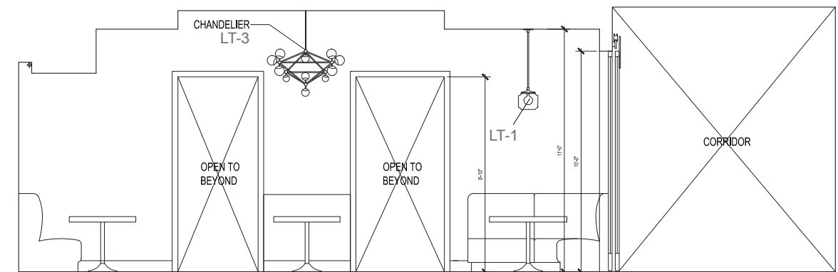
ELEVATION-VIEW TOWARD DINING ZONE 1
