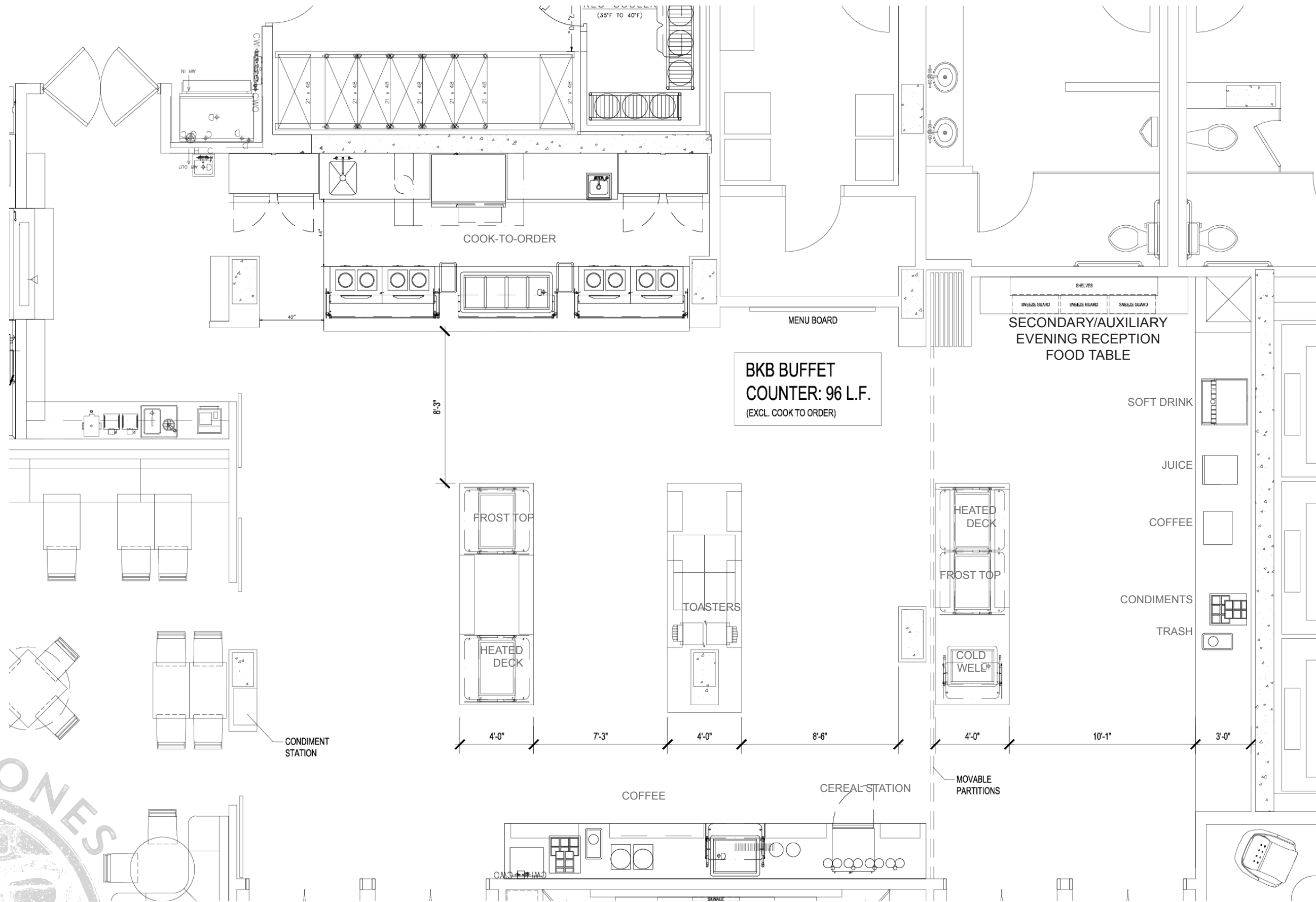
BKB BUFFET - FLOOR PLAN
