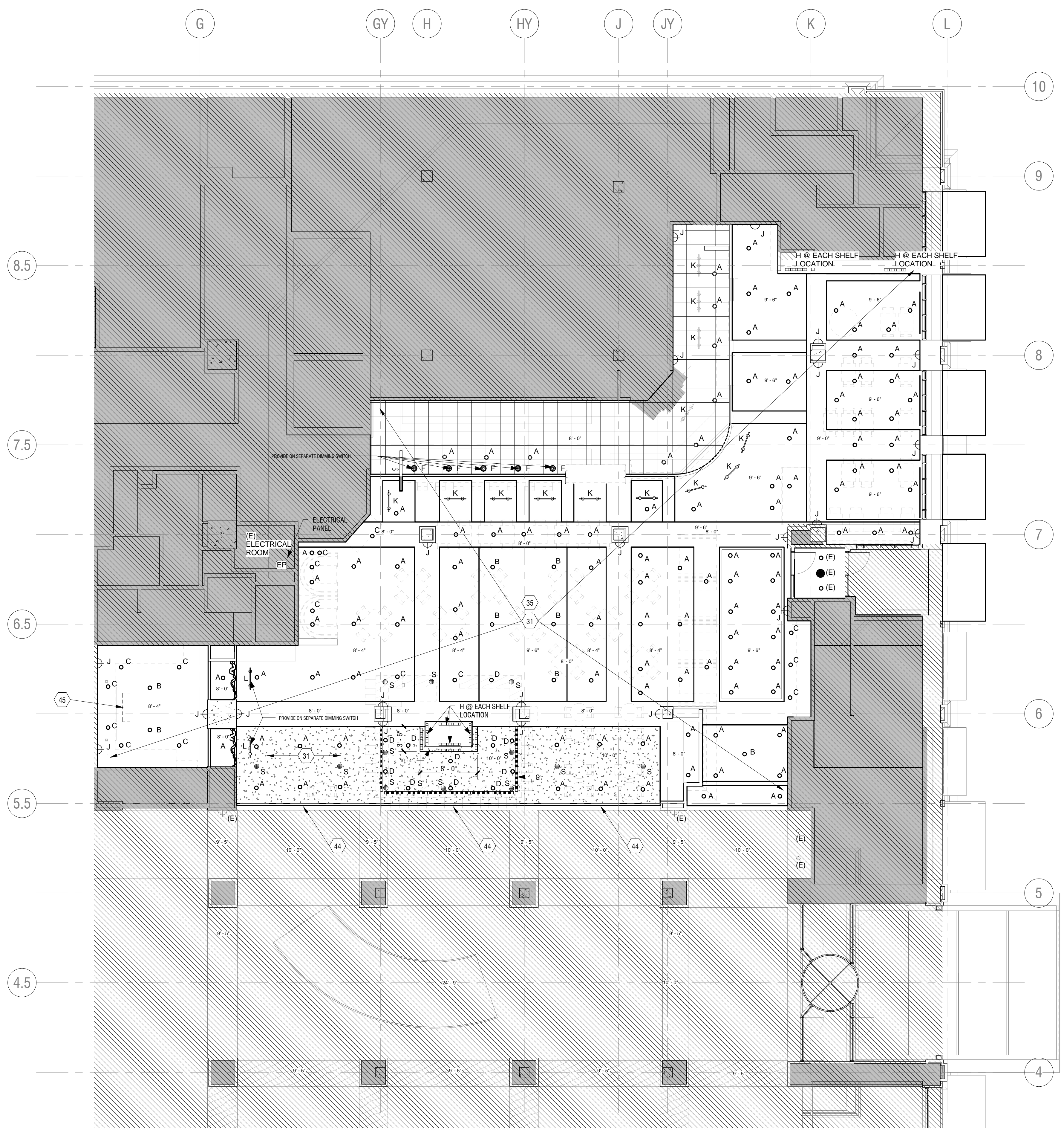
PROPOSED REFLECTED CEILING PLAN 1 1/8" = 1'-0"
