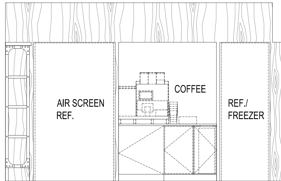
ELEVATION -VIEW TOWARD COFFEE STATION
