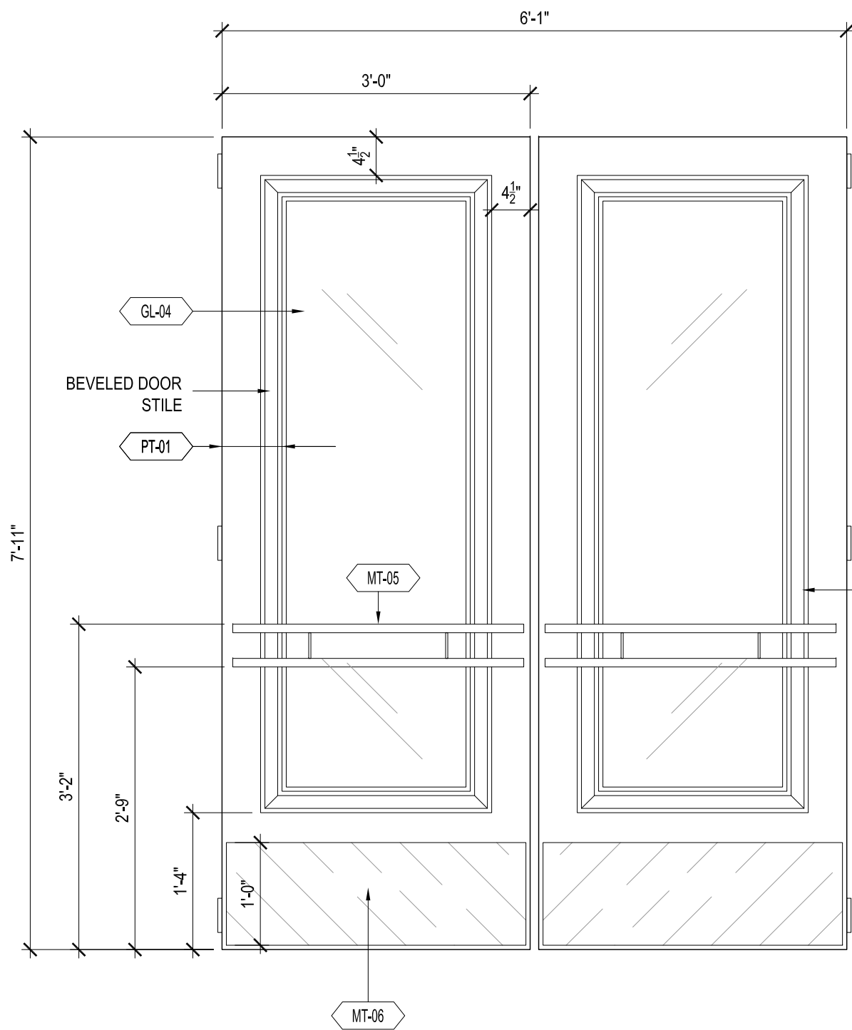
DOOR DESIGN CLOSEUP | SCALE: 3/4" = 1'-0"
