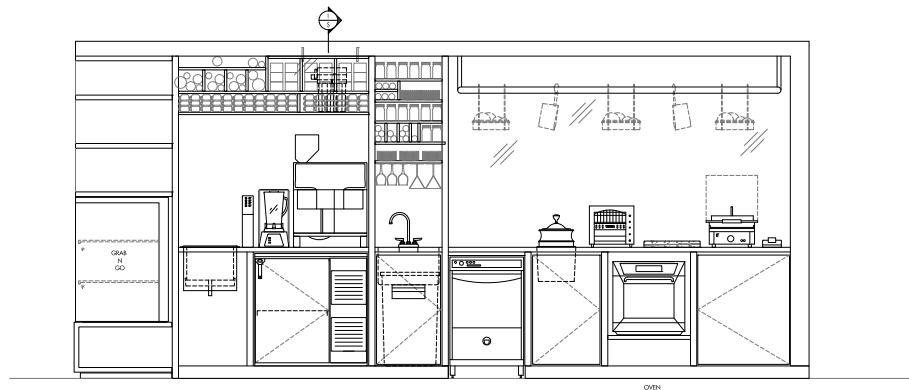
TIER I OPEN ELEVATION
