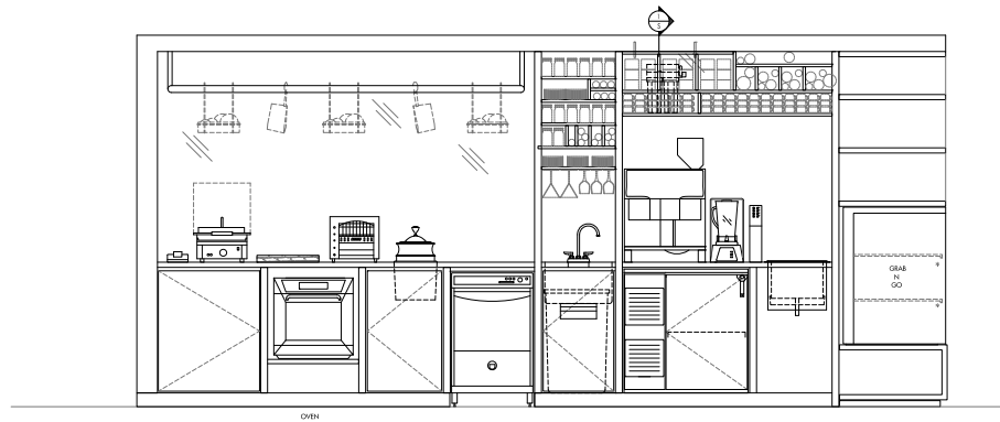
TIER I OPEN ELEVATION
