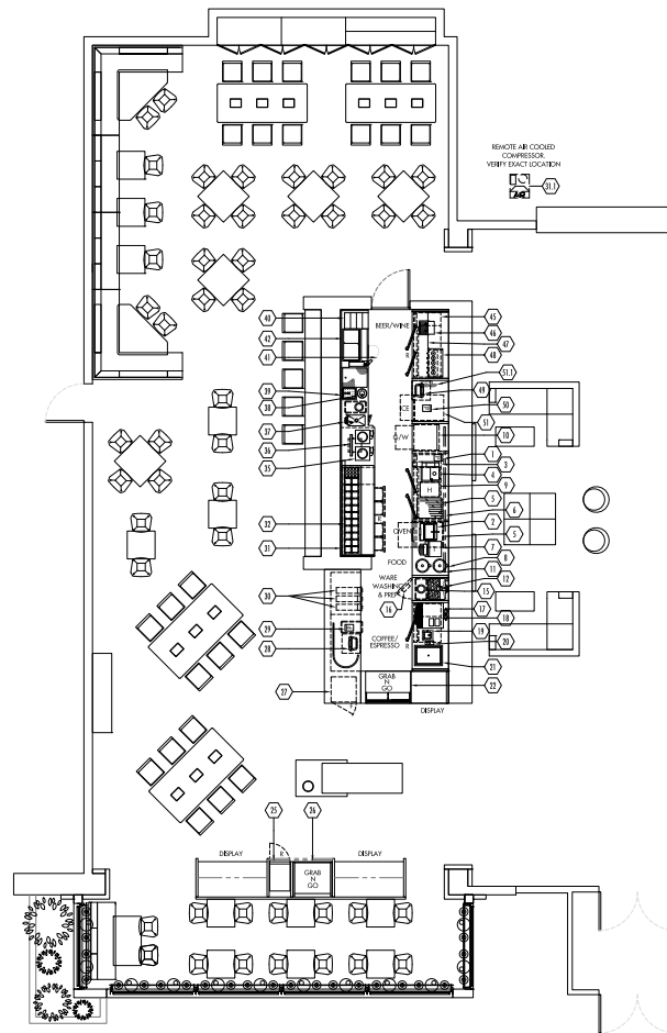
TIER 1 FILTERED EQUIPMENT FLOOR PLAN (W/ ADDITIONAL OPTIONS)
