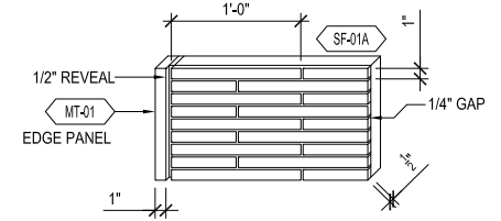
TILE PATTERN DETAILS | SCALE: NTS
