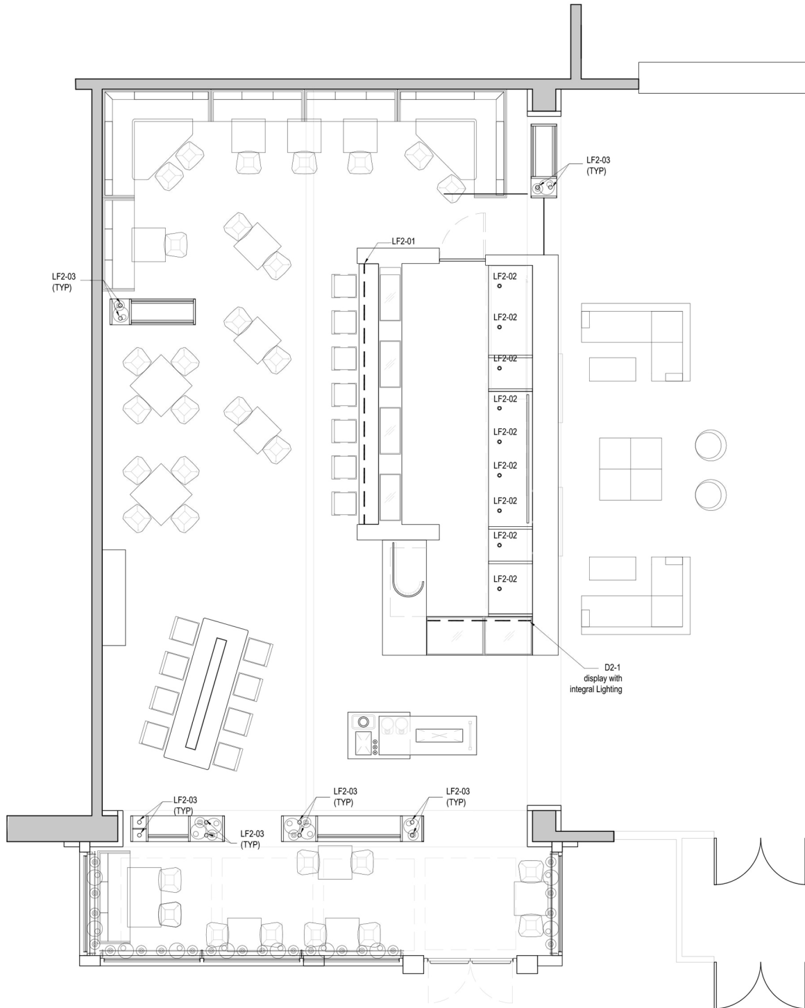
OPTION A MILLWORK LIGHTING | SCALE 1/4" = 1'-0"
