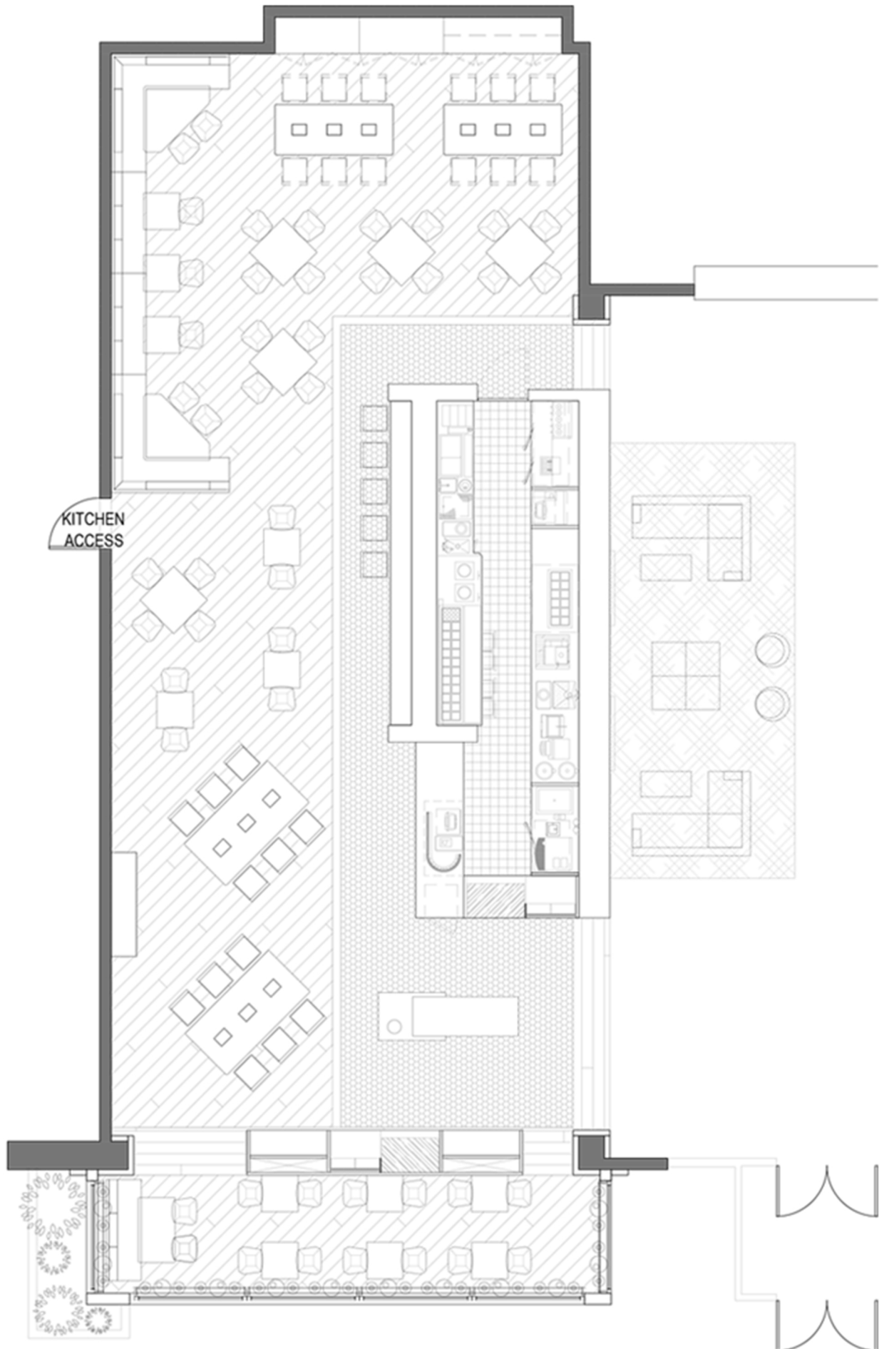
MARKET T1 FILTERED FLOORPLAN (W/ ADDITIONAL OPTIONS) | SCALE: 1/8" = 1'-0" SEATING COUNT: 77 + 12 ADDITIONAL AT BUFFET (NOT INCL. LIVING ROOM)
