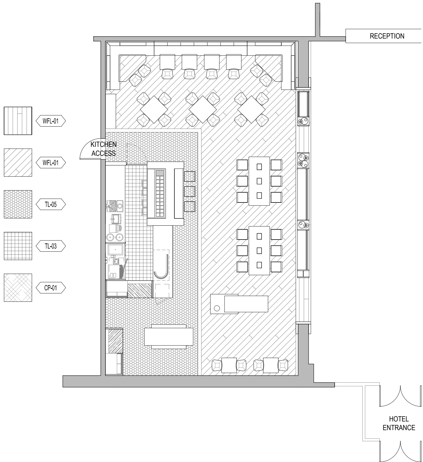
MARKET T1 OPEN FLOORPLAN (STANDARD) | SCALE: 1/8" = 1'-0" SEAT COUNT: 51
