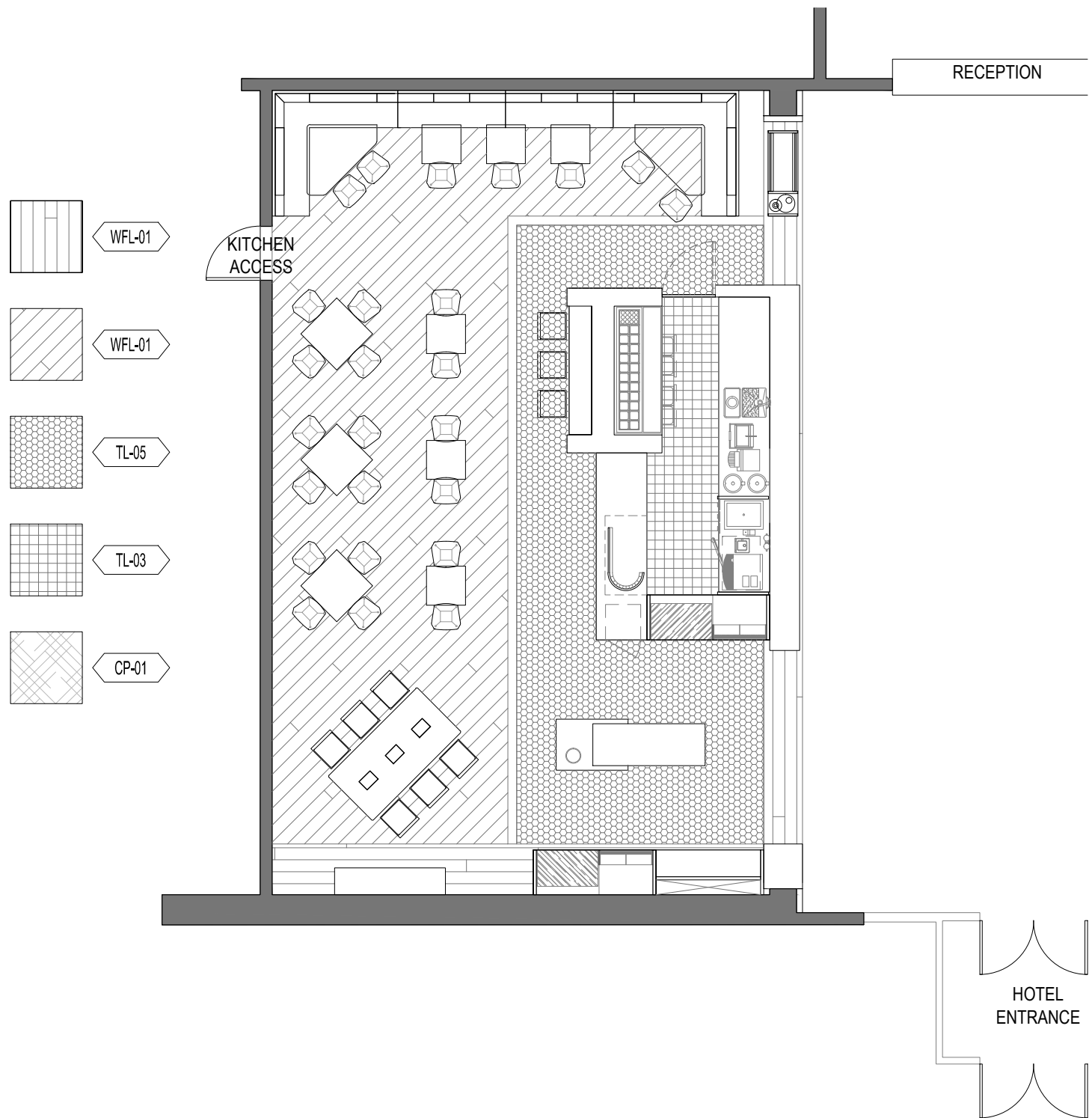
MARKET T1 FILTERED FLOORPLAN (STANDARD) | SCALE: 1/8" = 1'-0" SEAT COUNT: 45
