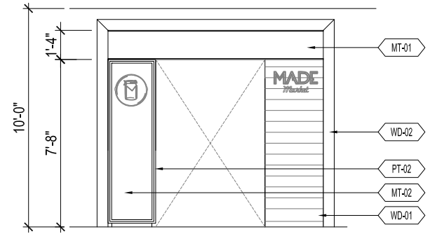
STOREFRONT ELEVATION
