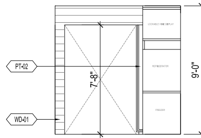
PORTAL ELEVATION
