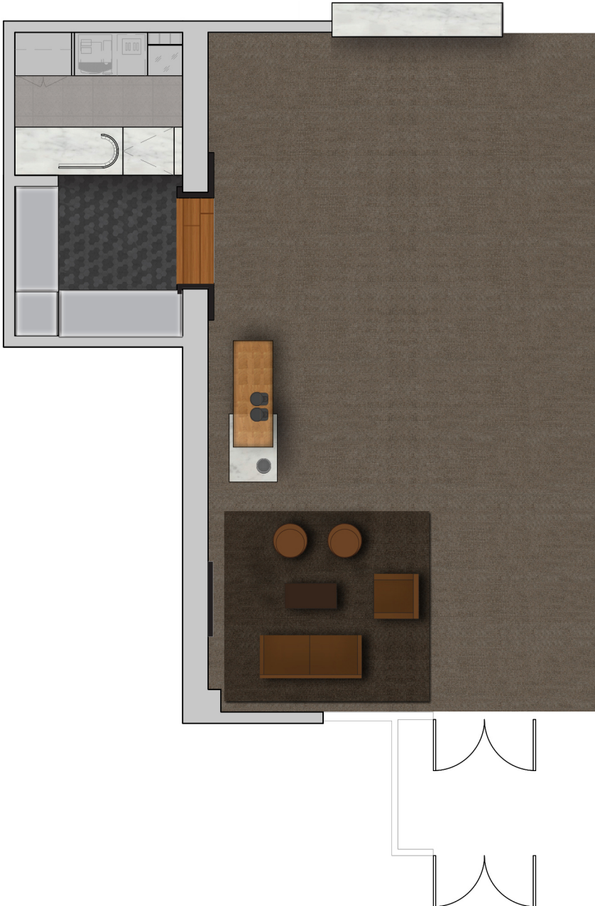
MARKET T2 FLOORPLAN (W/ ADDITIONAL OPTIONS) | SCALE: 1/8" = 1'-0"
